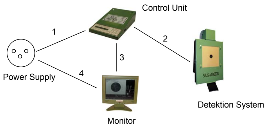
Figure 1 Minimal Cabling
